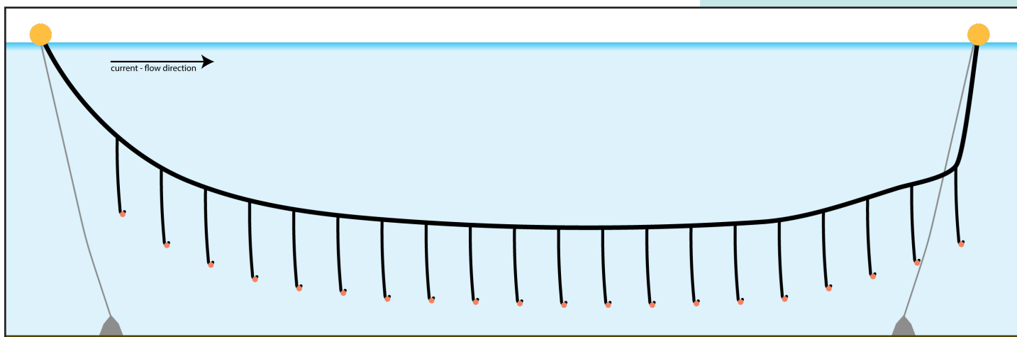
Set-line diagram.
